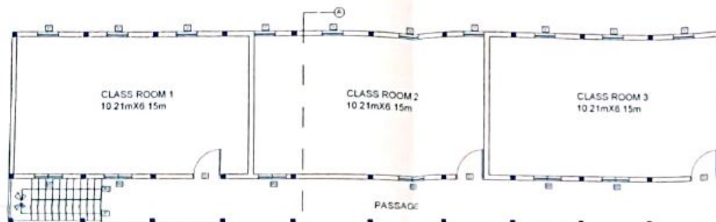
FIRST FLOOR FLOOR PLAN
